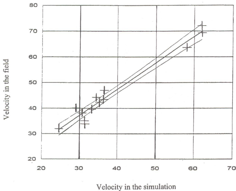
Figure 7: Real-life driving velocities vs. simulator driving velocities ( r = .982 ; Regression: (\text{real-life}) \text{ speed} = 6.48 + 1.02 * \text{simulatorspeed} )
