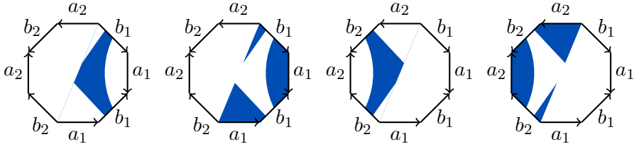
FIGURE 2. The open cover of \Sigma in Example 1.4
