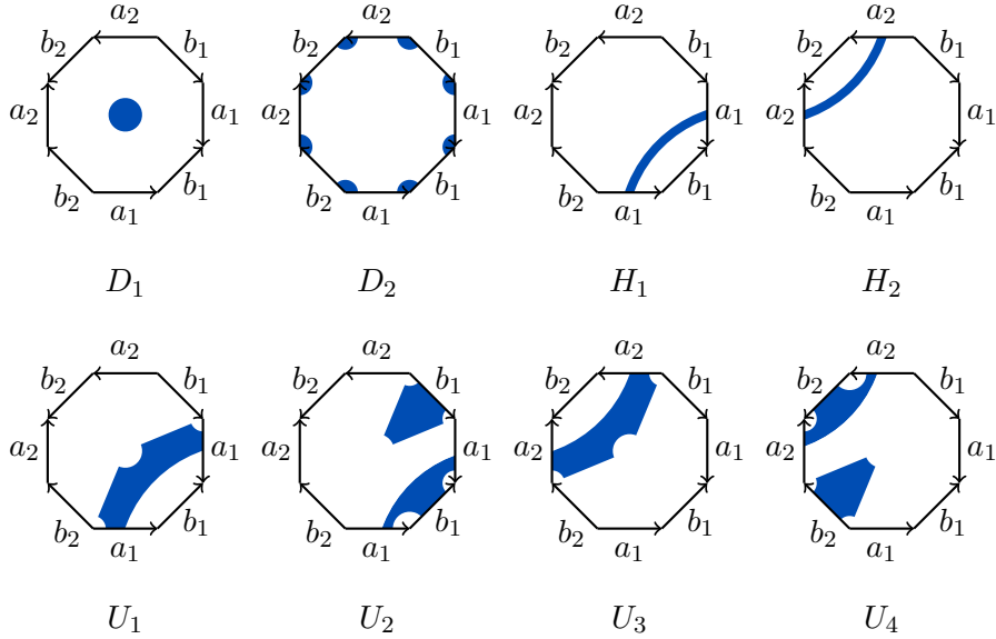
FIGURE 1. The open cover of \Sigma in Example 1.3
